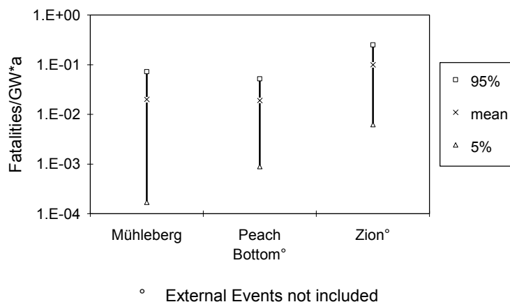
Fig. 7.2.9 Estimated latent cancer fatalities due to hypothetical severe accidents (per GWe*a) for the Swiss nuclear power plant Mühleberg and two US plants.
