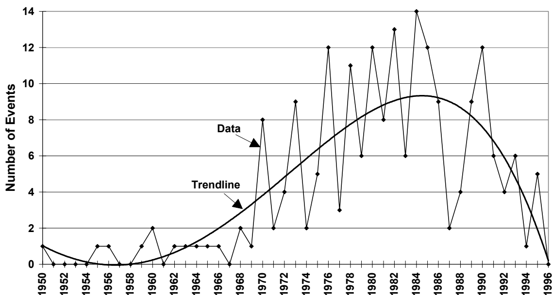
Fig. 6.4.7 World-wide number of severe ( \geq 5 fatalities) gas accidents.
